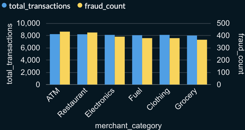
Fraud by merchant category
